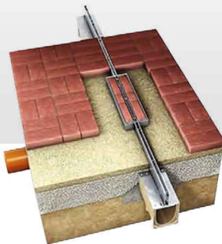
BrickSlot T
