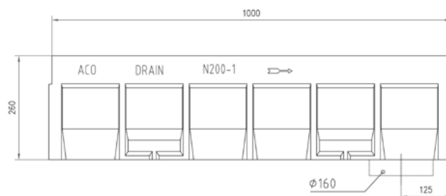
Canal N200 H26
