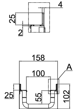
Detalle A (2:1)
