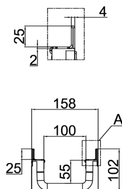
Detalle A (2:1)
