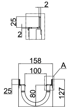
Detalle A (2:1)
