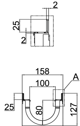
Detalle A (2:1)
