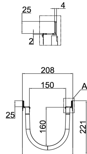
Detalle A (2:1)
