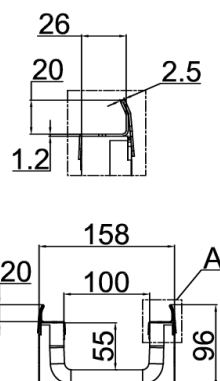
Detalle A (2:1)
