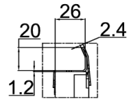
Detalle A (2:1)
