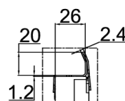
Detalle A (2:1)
