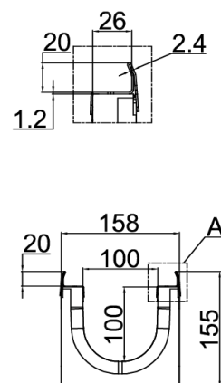
Detalle A (2:1)
