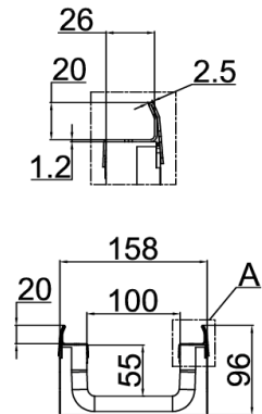
Detalle A (2:1)
