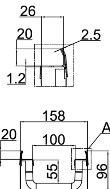
Detalle A (2:1)
