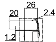
Detalle A (2:1)
