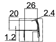
Detalle A (2:1)
