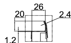
Detalle A (2:1)
