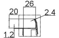
Detalle A (2:1)
