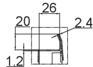
Detalle A (2:1)
