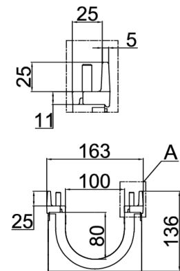
Detalle A (2:1)
