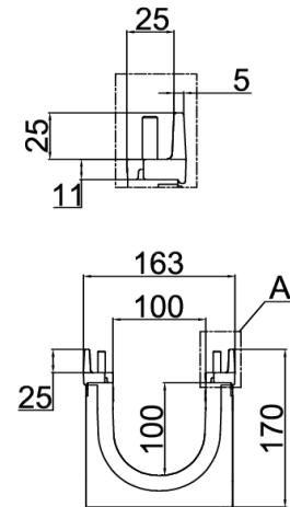
Detalle A (2:1)
