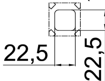
Detalle A (2:1)
