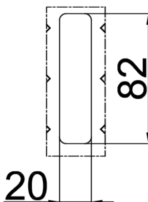
Detalle A (2:1)
