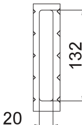
Detalle A (2:1)
