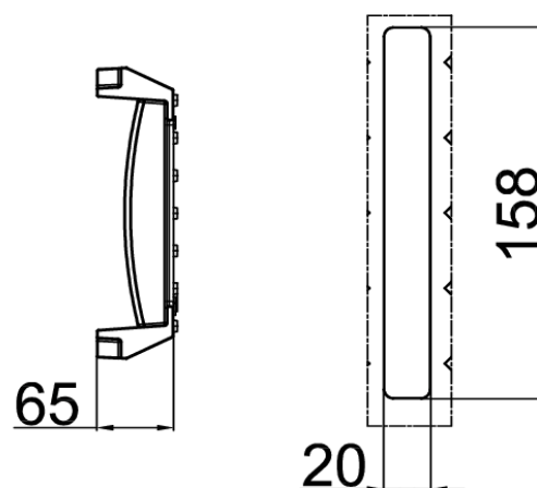
Detalle A (2:1)
