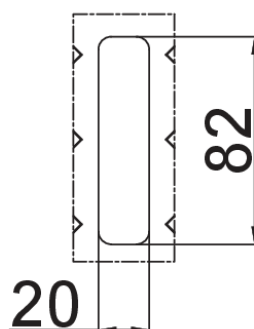
Detalle A (2:1)
