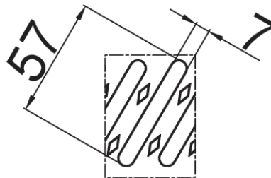
Detalle A (2:1)
