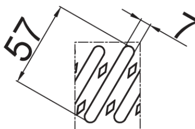
Detalle A (2:1)
