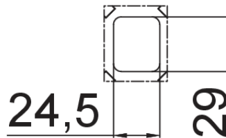
Detalle A (2:1)
