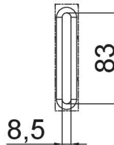
Detalle A (2:1)
