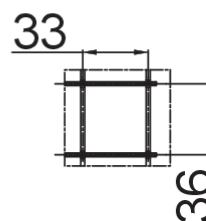
Detalle A (2:1)
