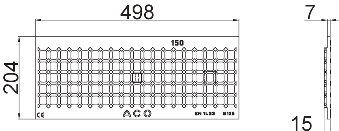
Detalle A (2:1)
