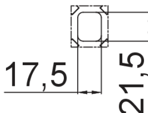
Detalle A (2:1)
