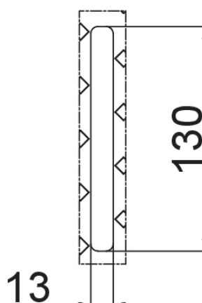
Detalle A (2:1)
