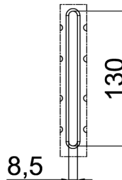
Detalle A (2:1)
