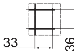
Detalle A (2:1)
