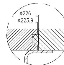
Detalle D E(5:1)
